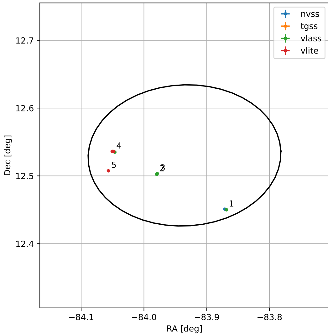
4FGL J1824.2+1231
