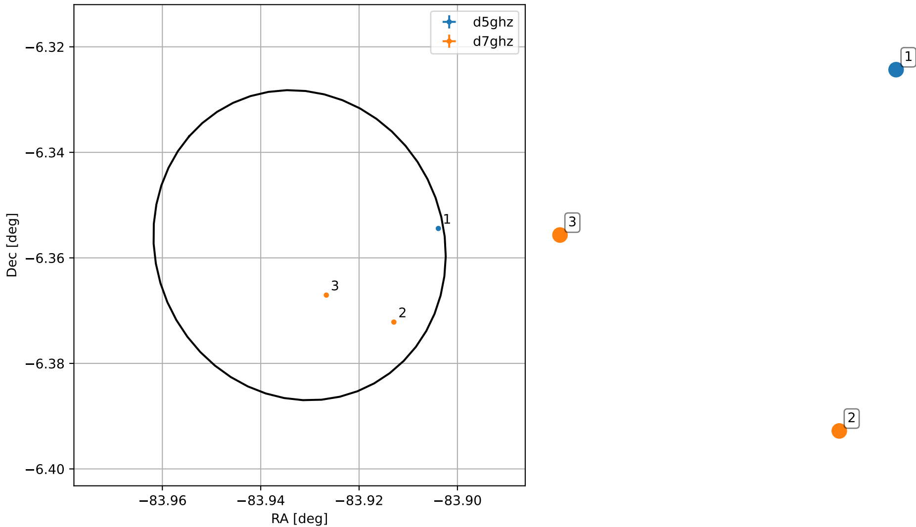
4FGL J1824.2-0621
