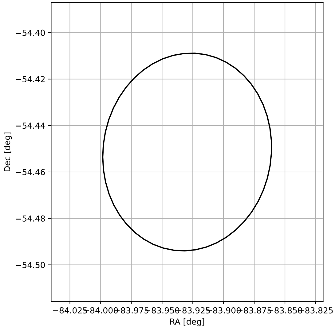
4FGL J1824.2-5427
