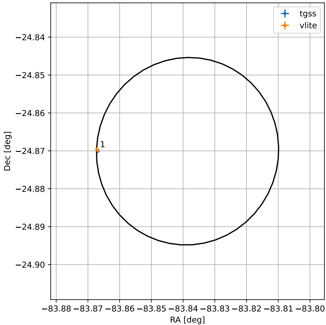
4FGL J1824.6-2452
