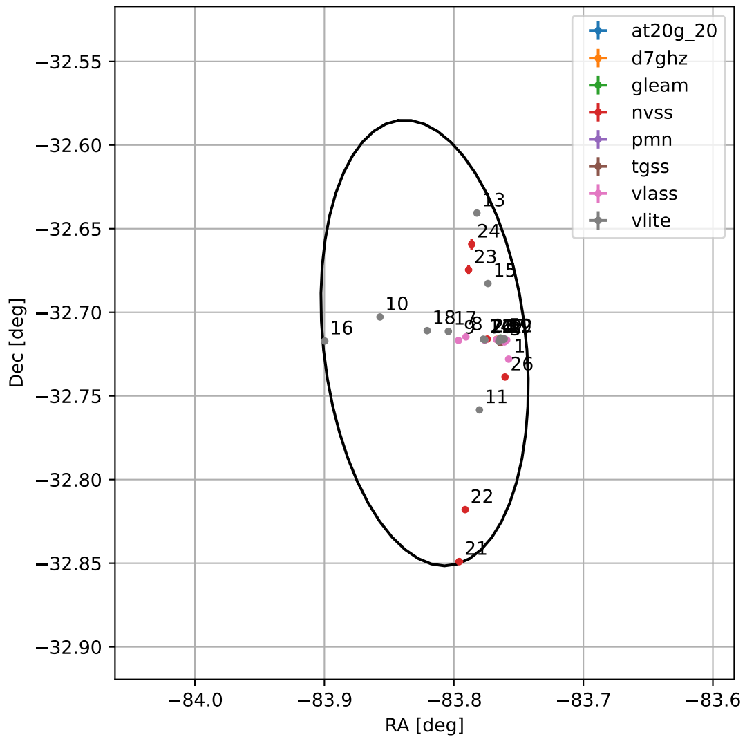
4FGL J1824.7-3243
