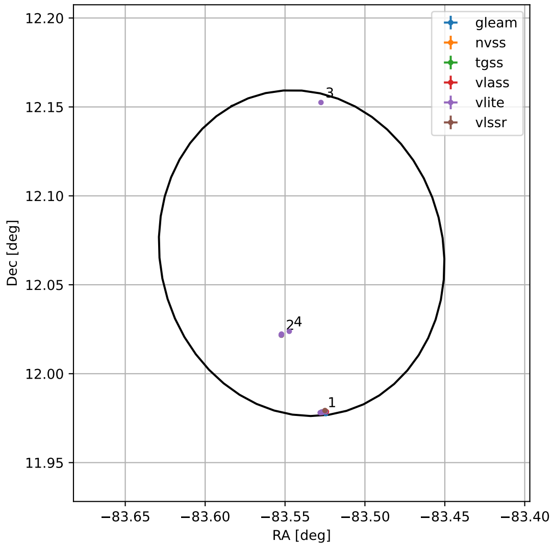
4FGL J1825.8+1204
