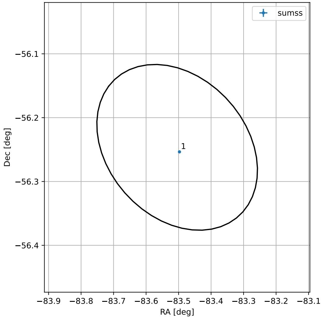
4FGL J1825.9-5614
