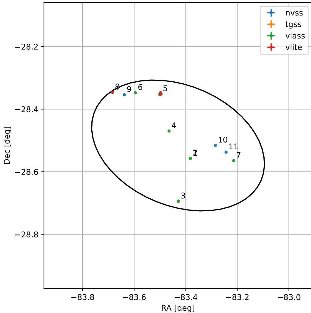
4FGL J1826.2-2830
