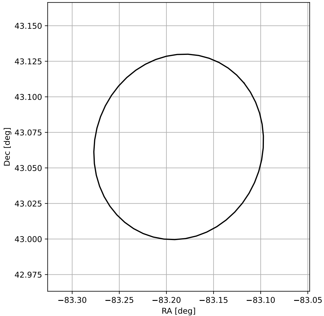
4FGL J1827.2+4303
