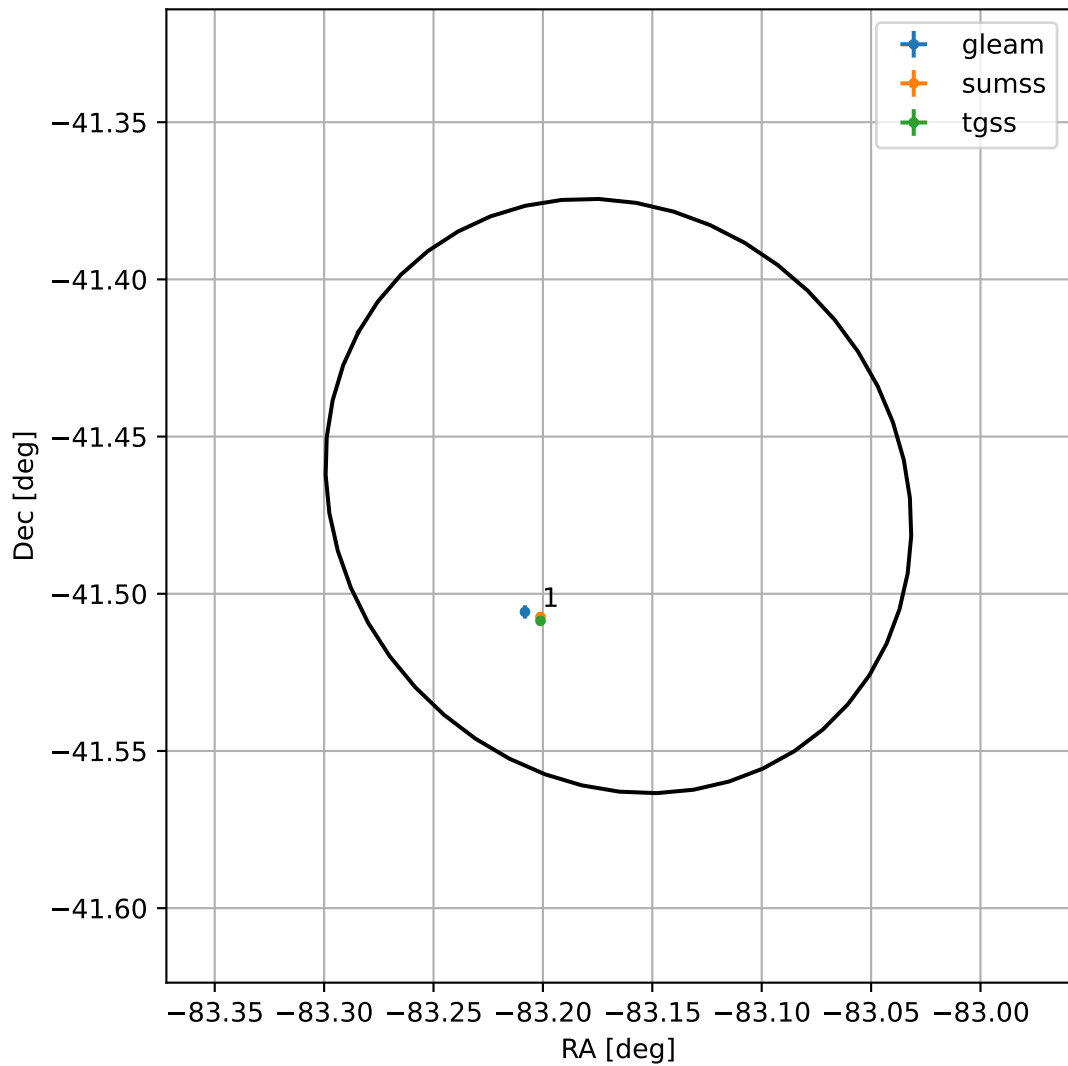
4FGL J1827.3-4128
