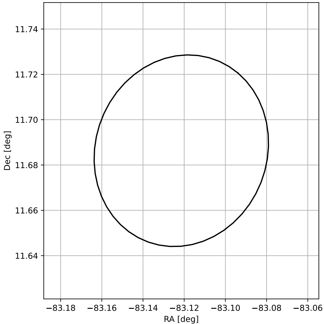
4FGL J1827.5+1141
