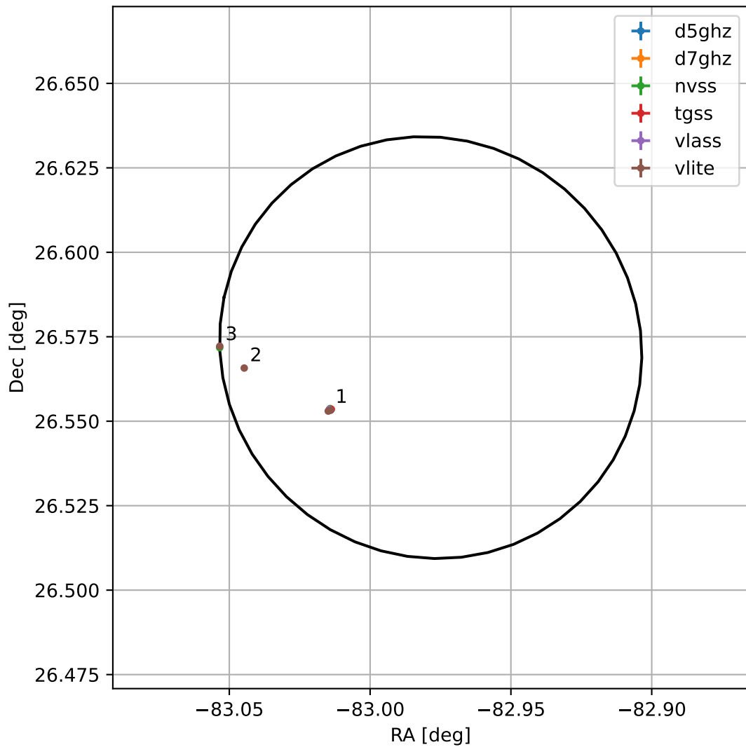
4FGL J1828.0+2634
