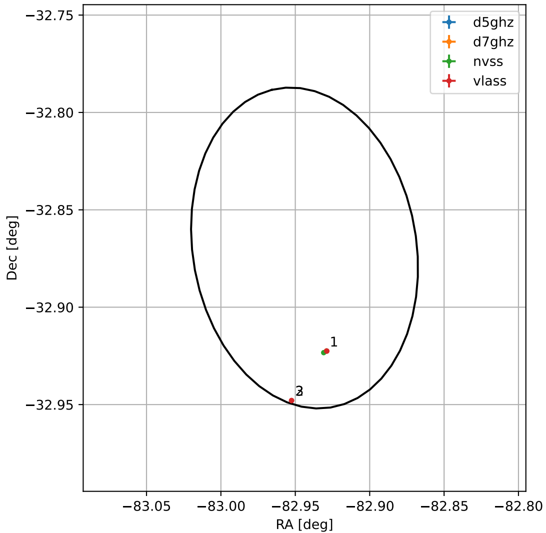
4FGL J1828.2-3252
