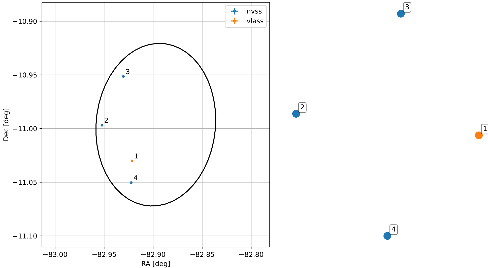
4FGL J1828.4-1059
