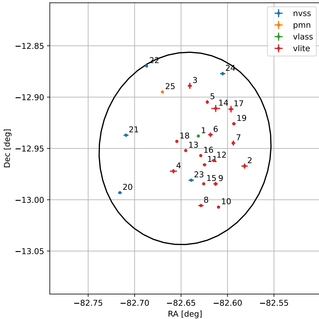
4FGL J1829.4-1256
