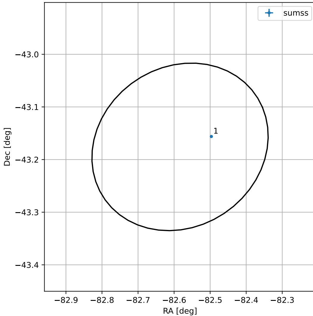
4FGL J1829.6-4310
