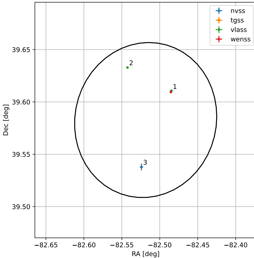
4FGL J1829.9+3934
