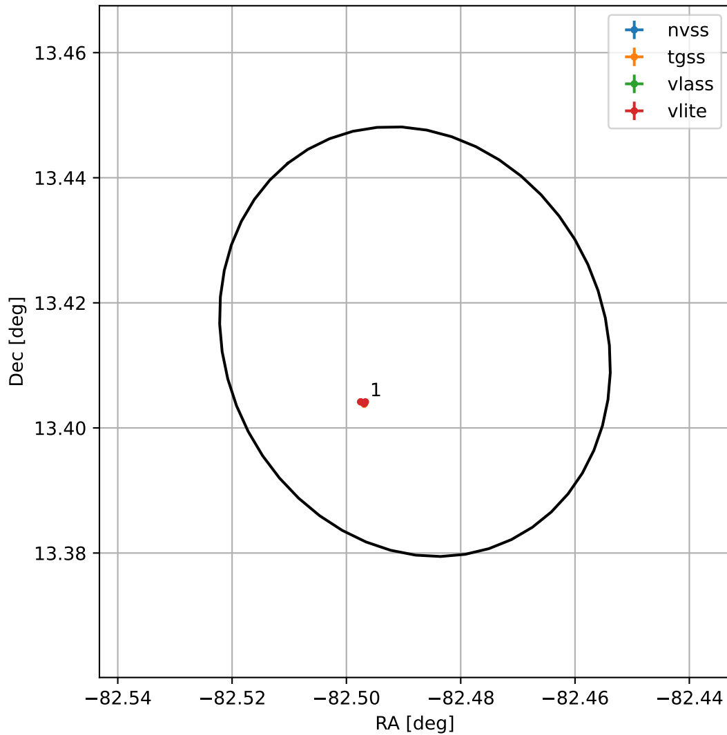
4FGL J1830.0+1324
