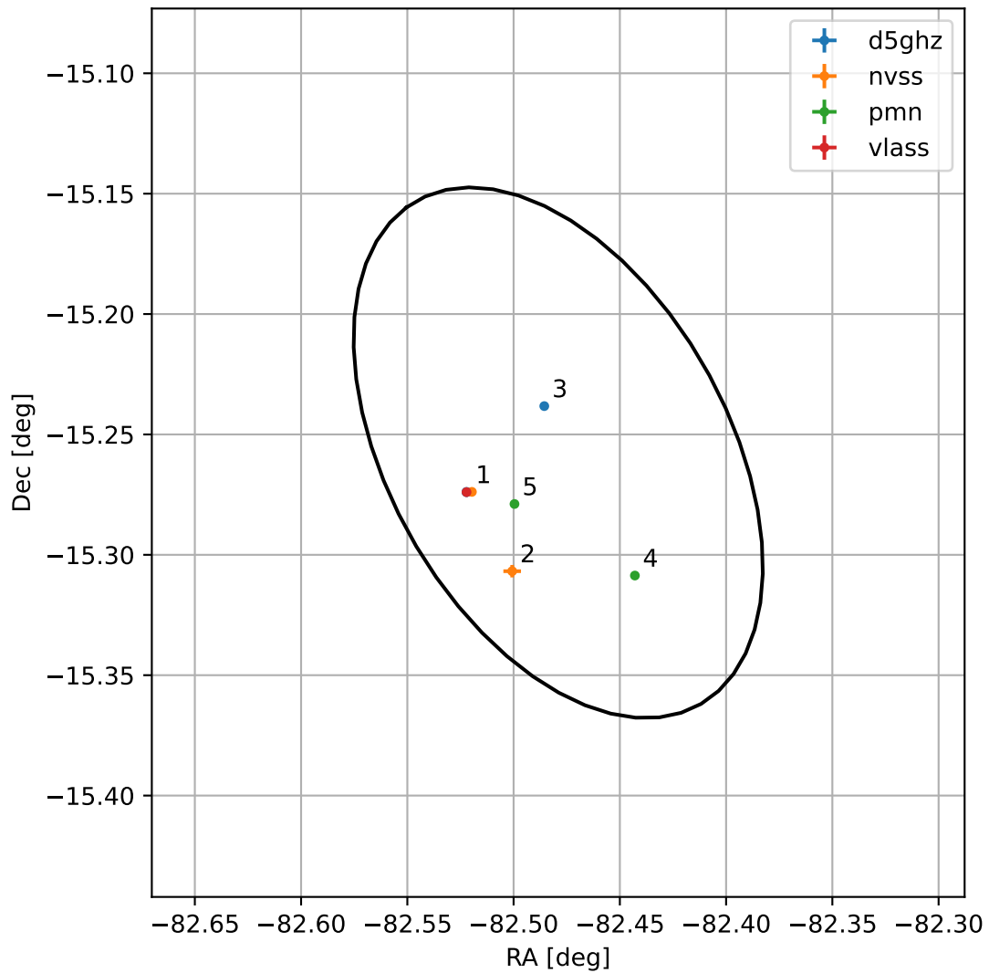
4FGL J1830.0-1515
