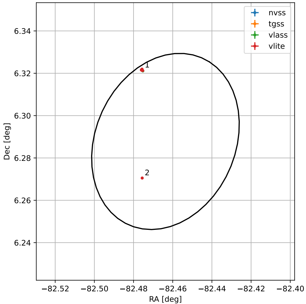
4FGL J1830.1+0617
