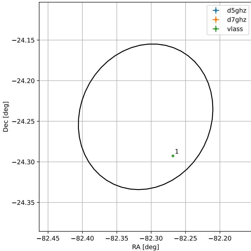
4FGL J1830.7-2414
