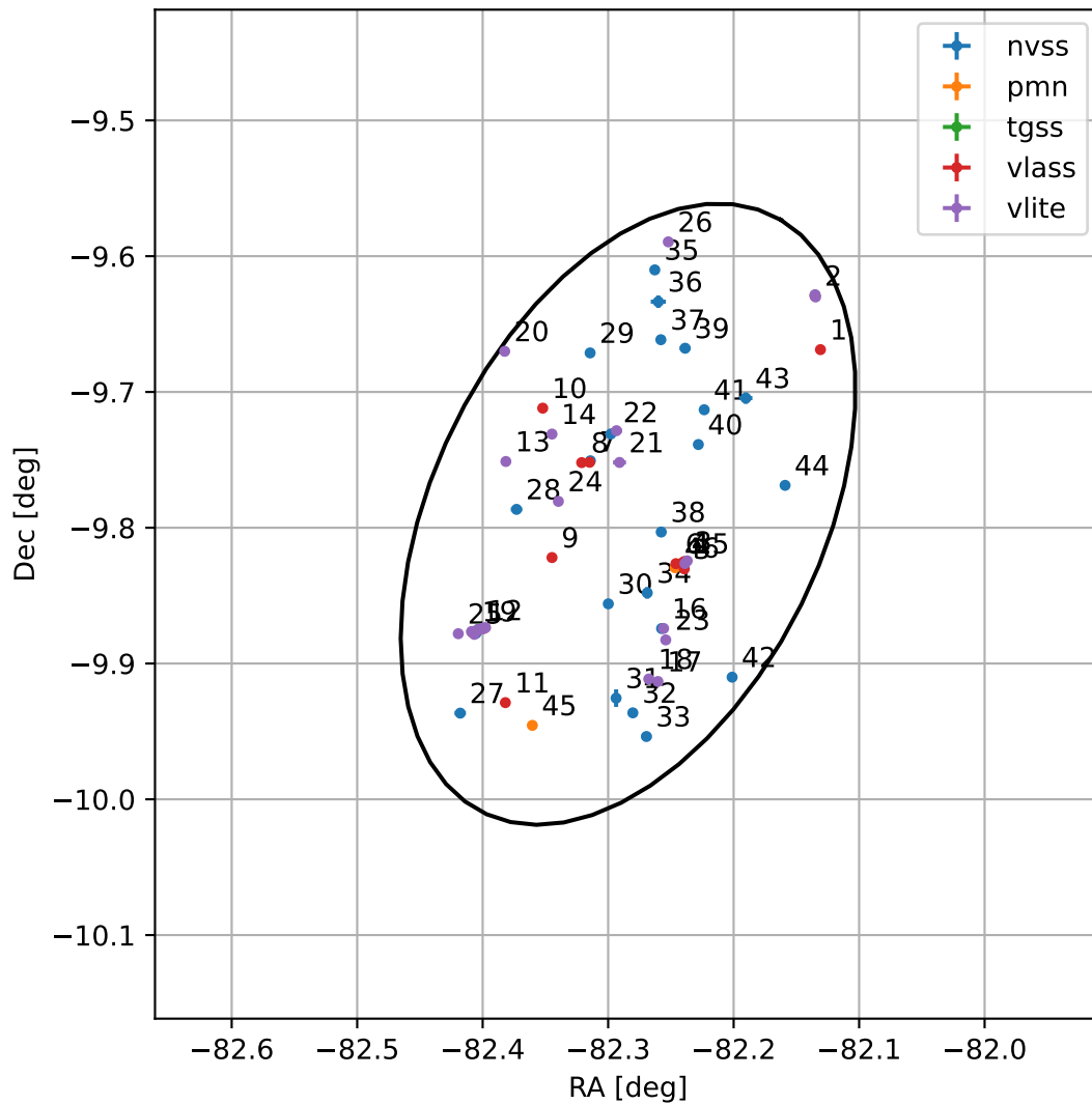
4FGL J1830.8-0947
