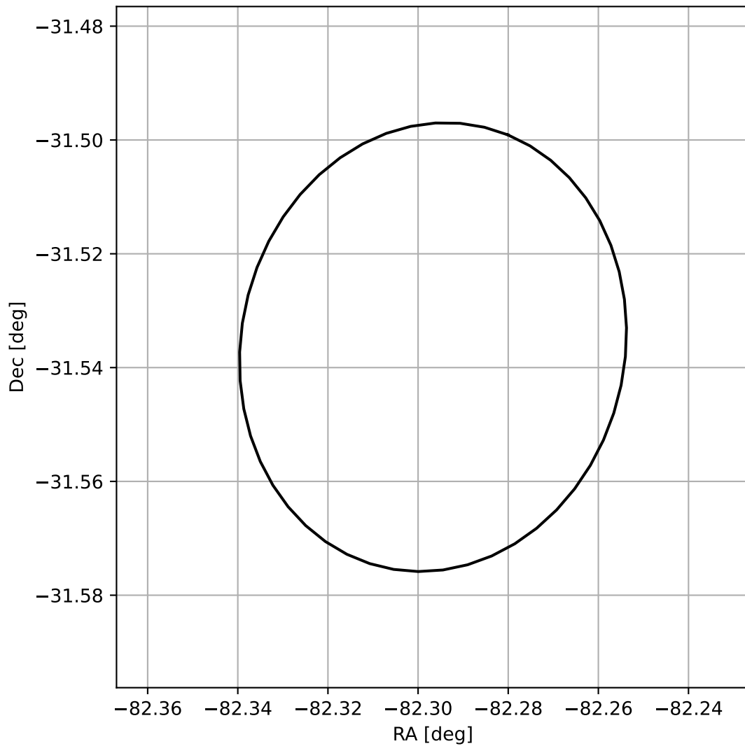
4FGL J1830.8-3132
