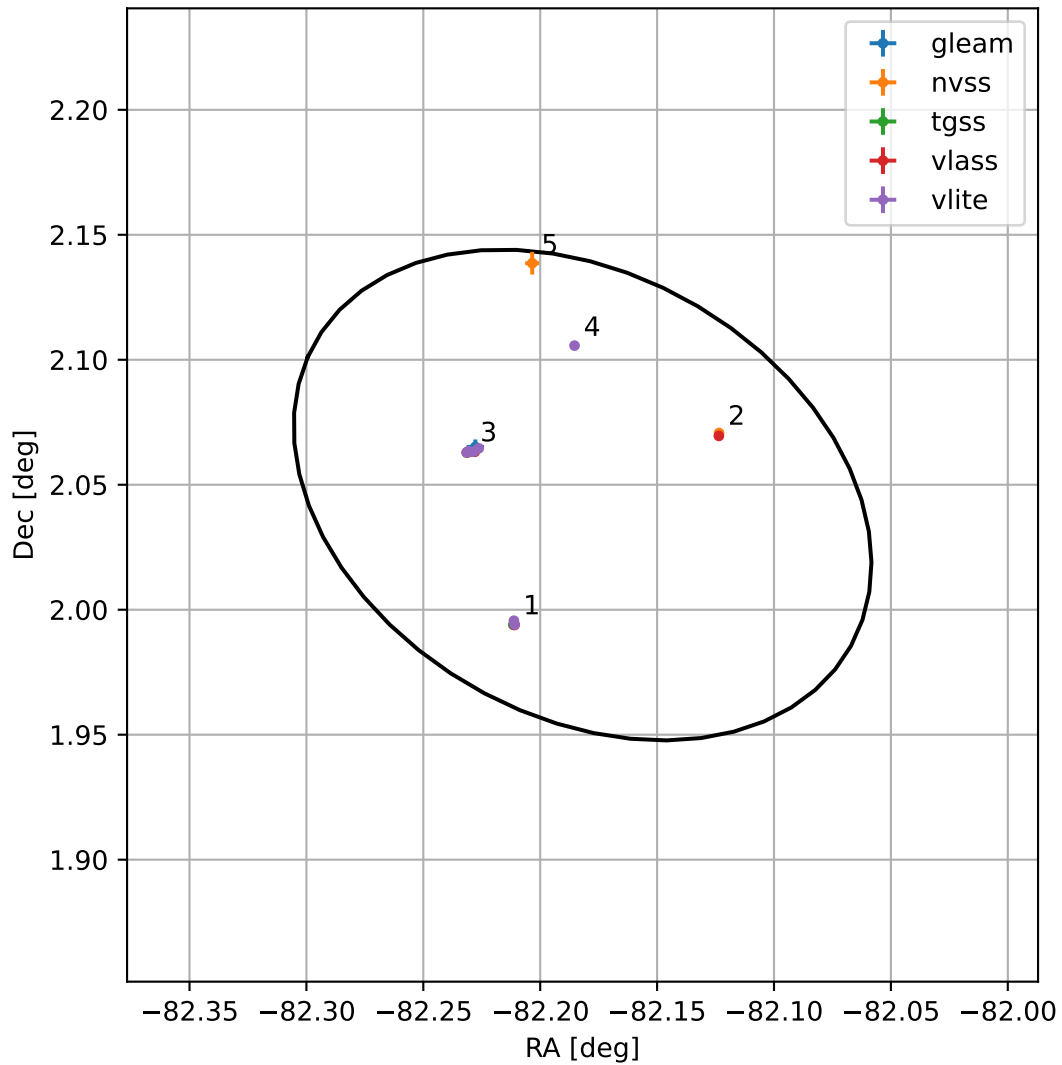
4FGL J1831.2+0202
