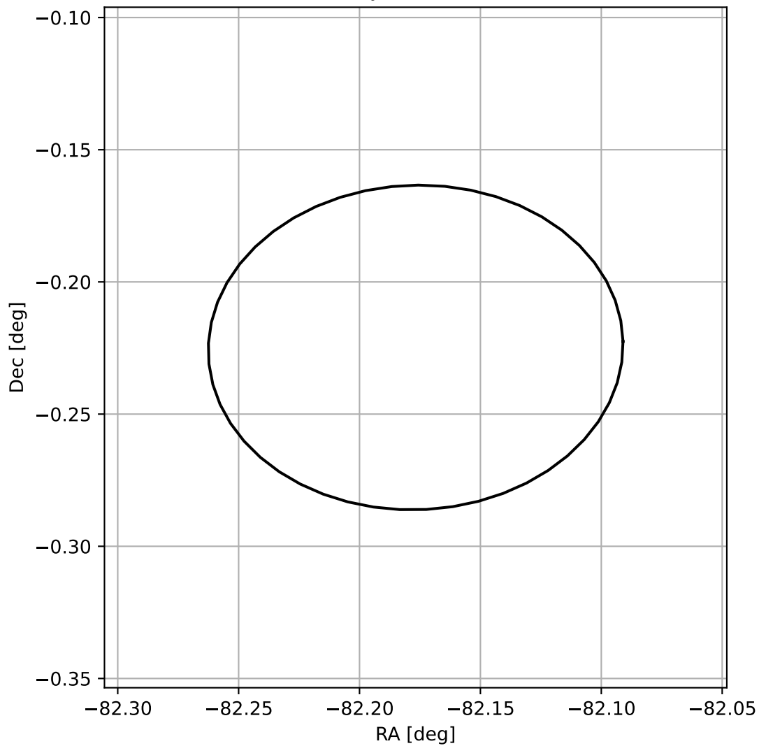
4FGL J1831.2-0013
