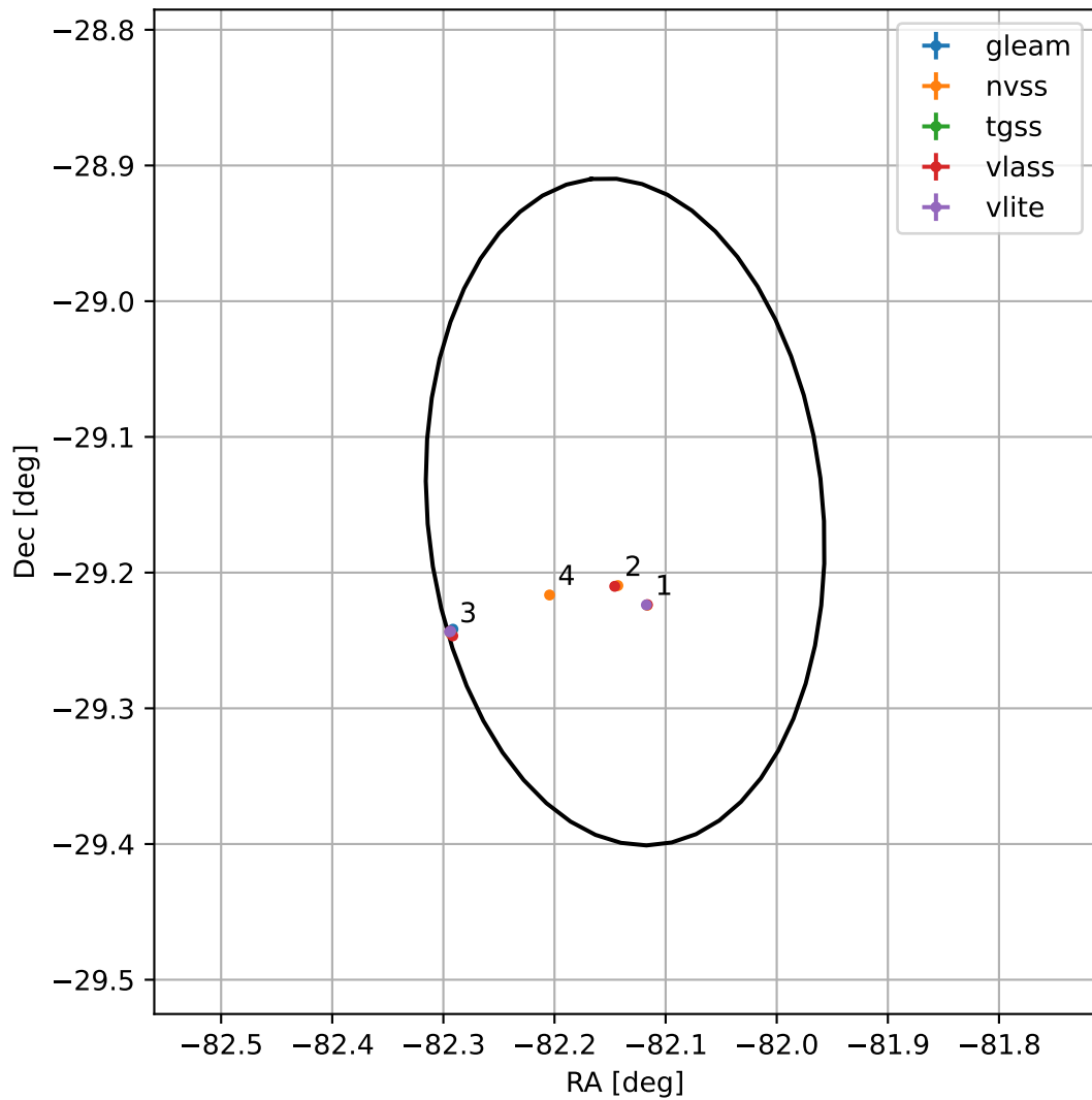
4FGL J1831.4-2909
