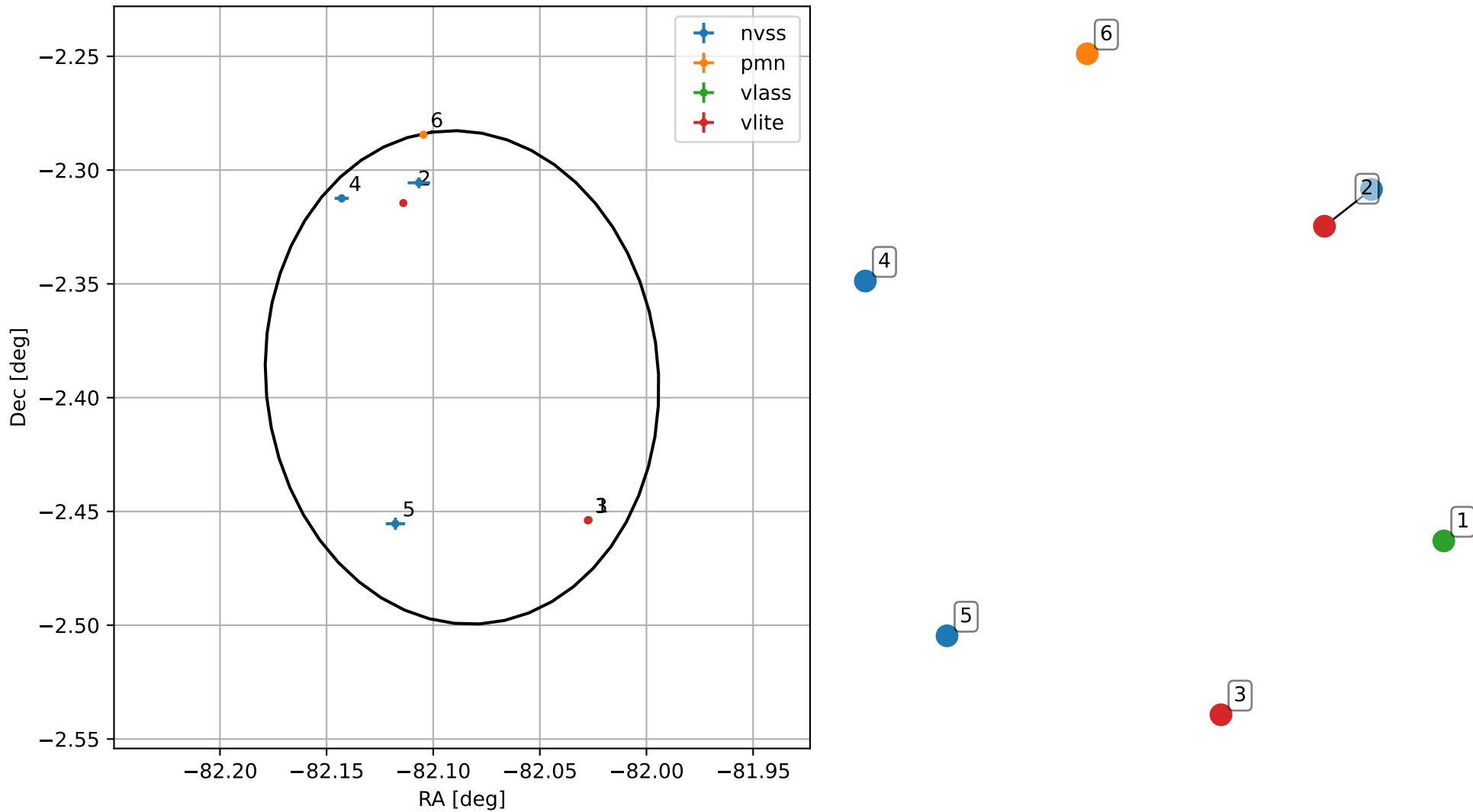
4FGL J1831.6-0223
