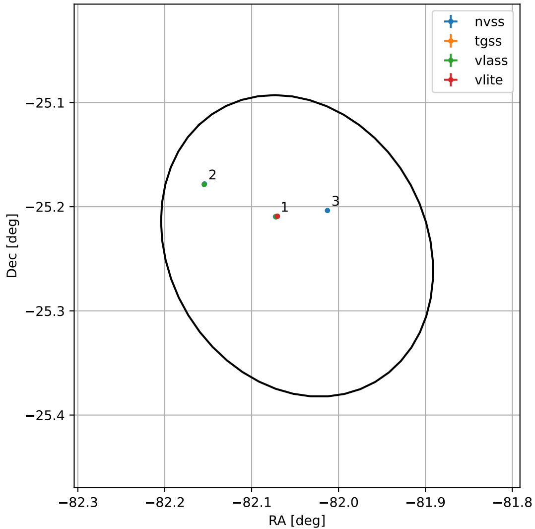
4FGL J1831.8-2514
