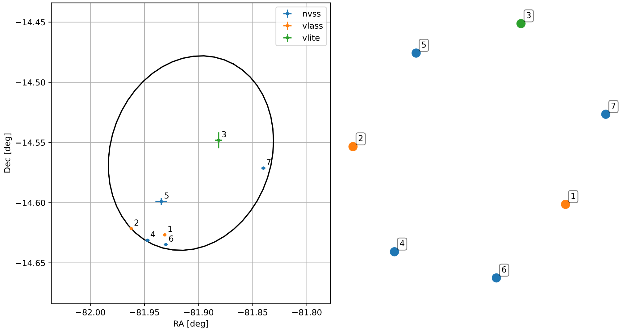
4FGL J1832.3-1433
