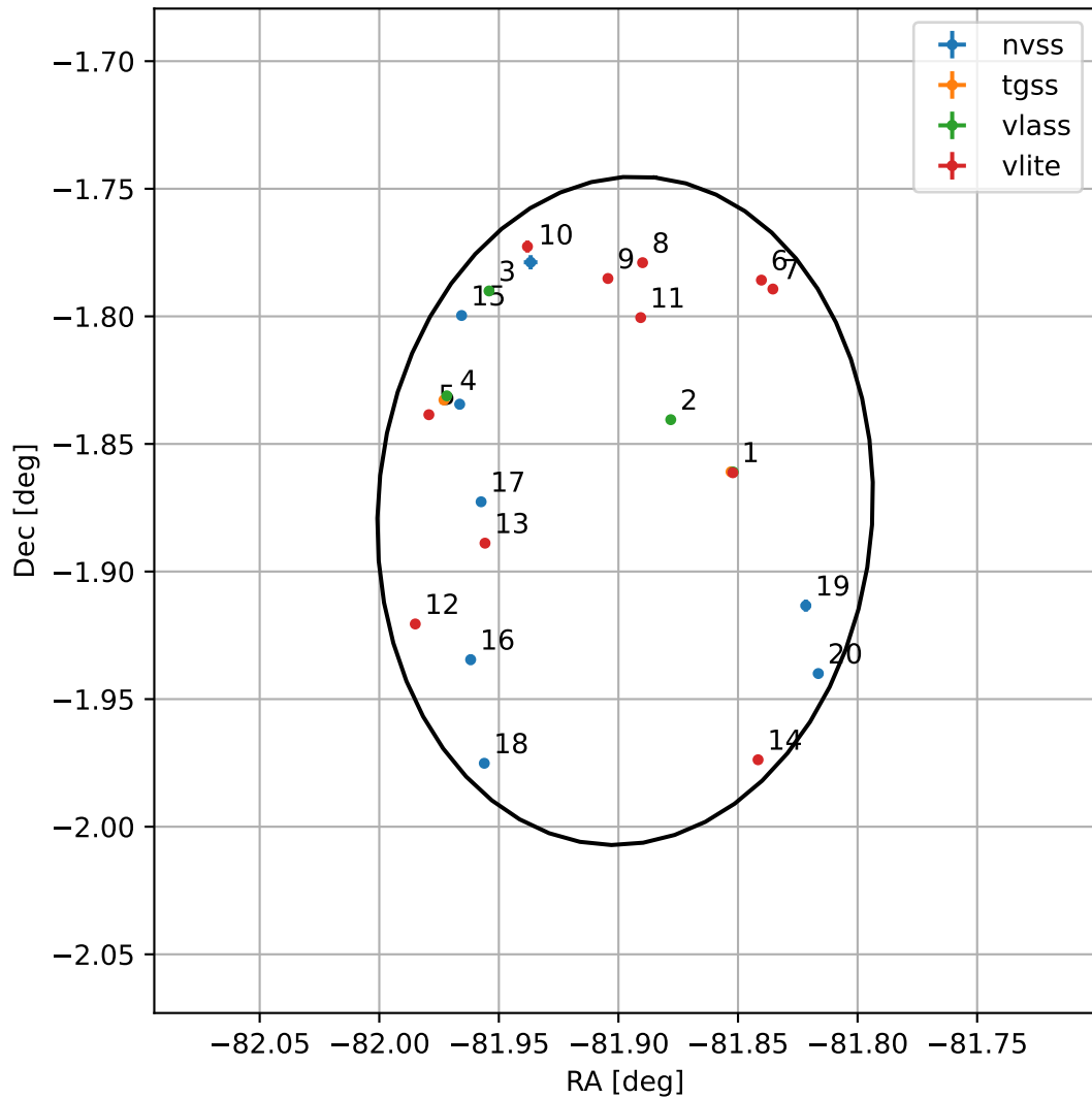
4FGL J1832.4-0152
