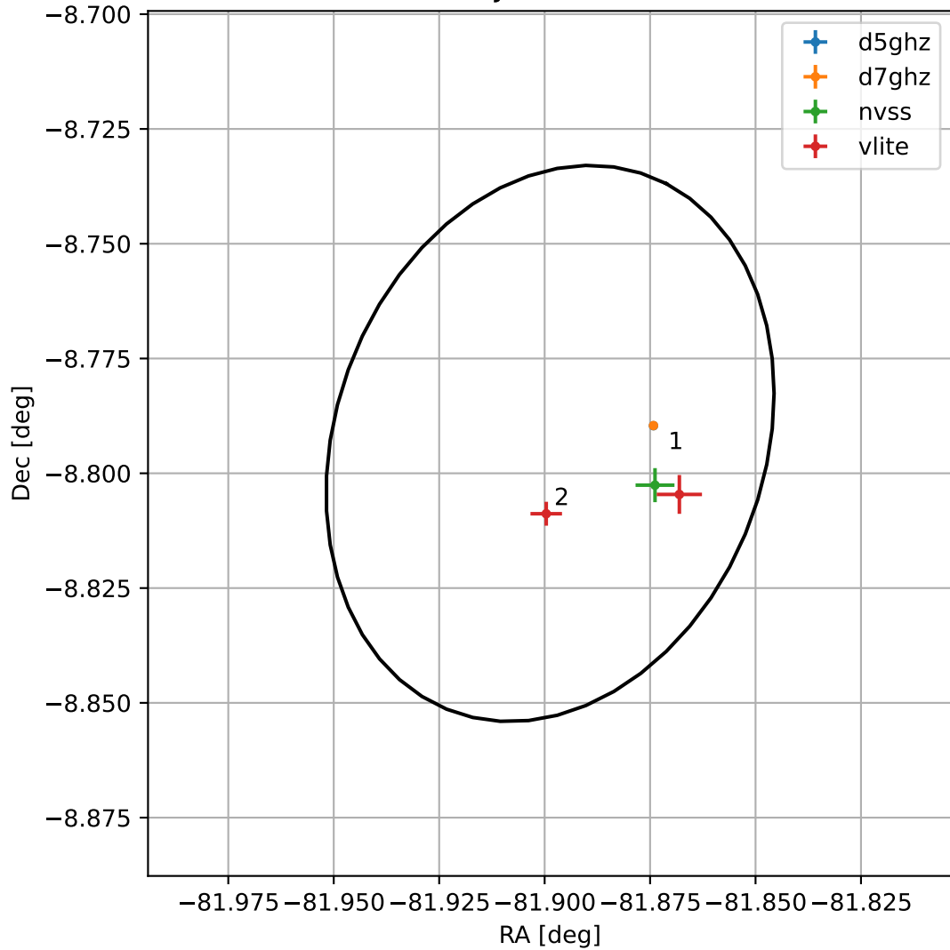
4FGL J1832.4-0847
