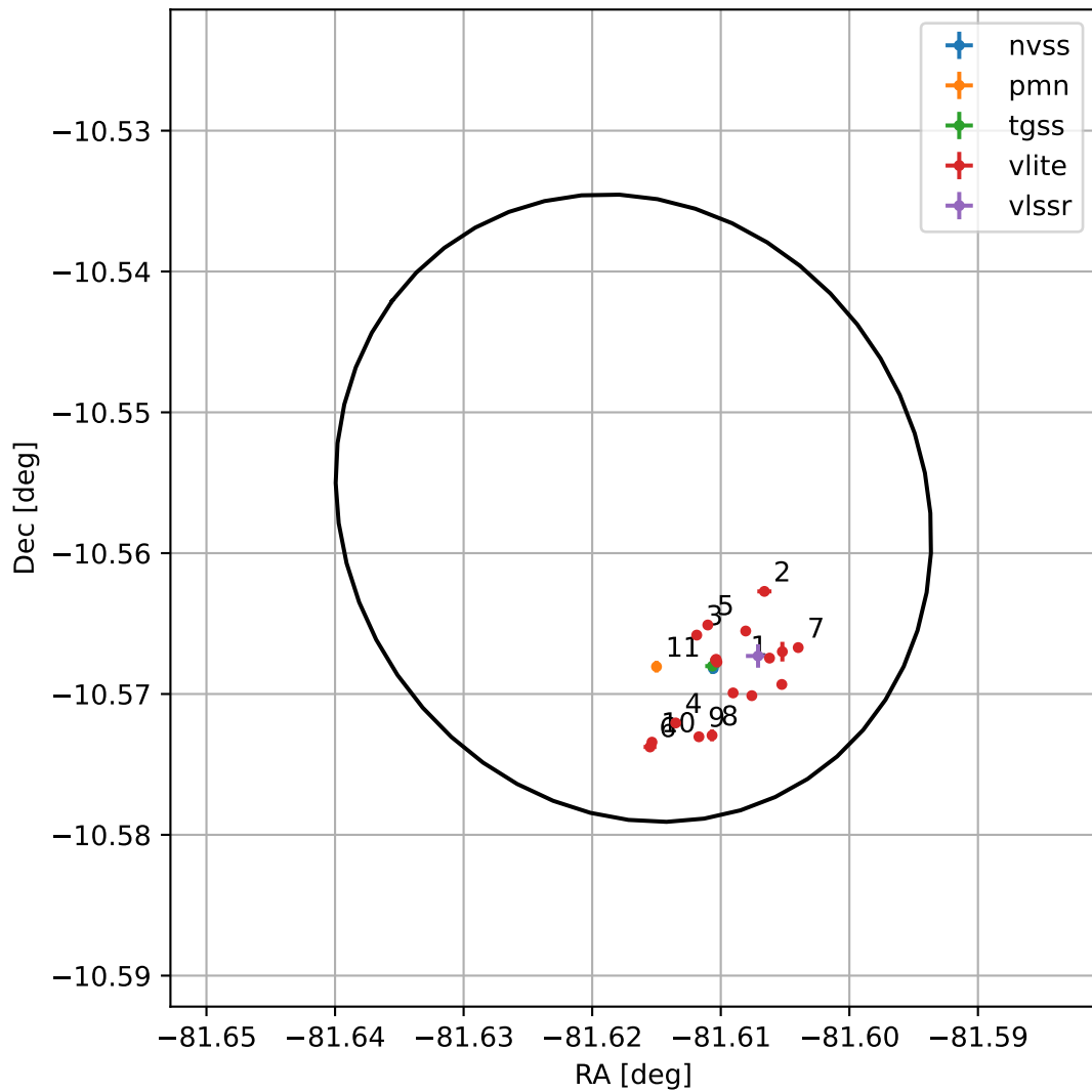
4FGL J1833.5-1033
