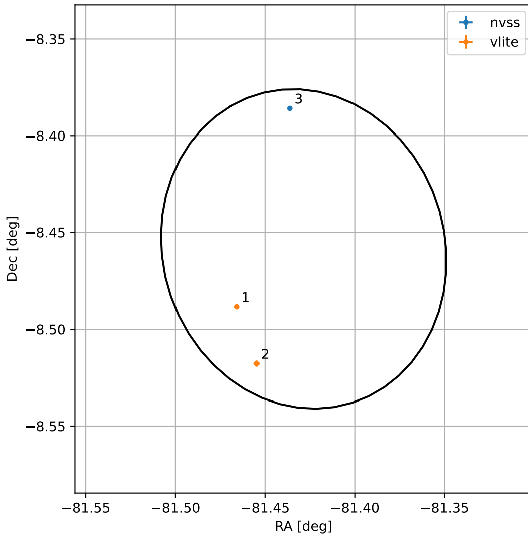
4FGL J1834.2-0827
