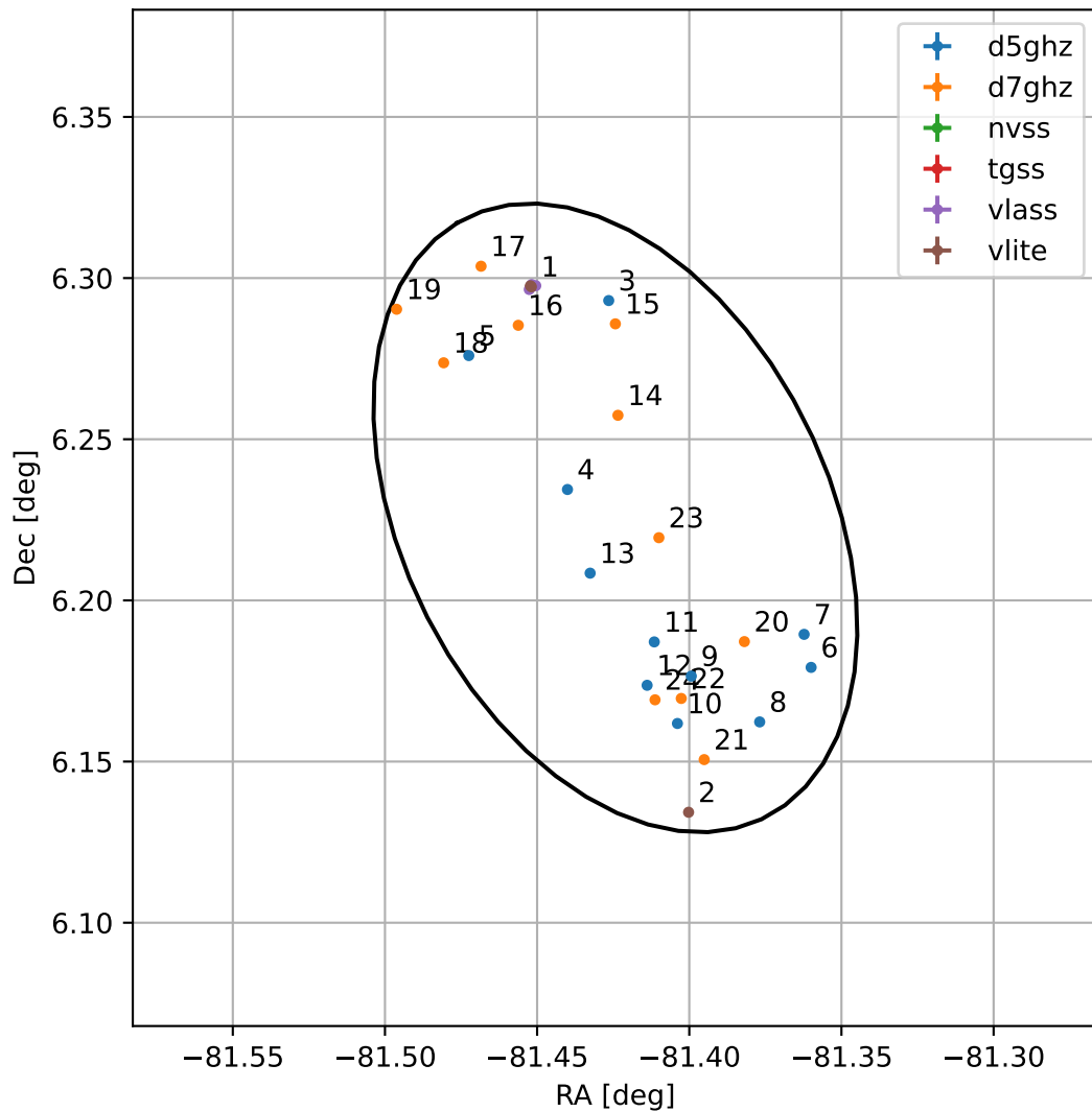
4FGL J1834.3+0613
