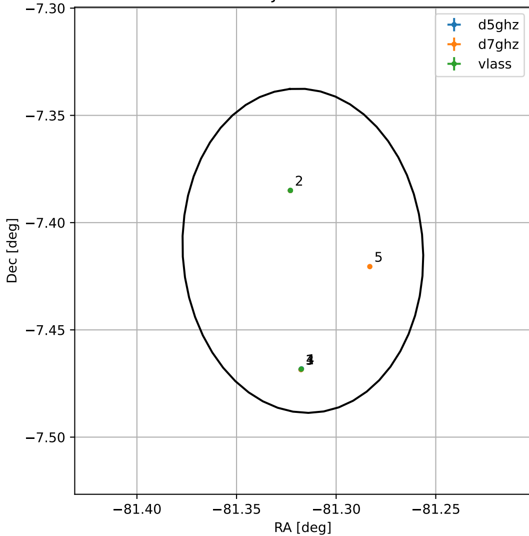
4FGL J1834.7-0724
