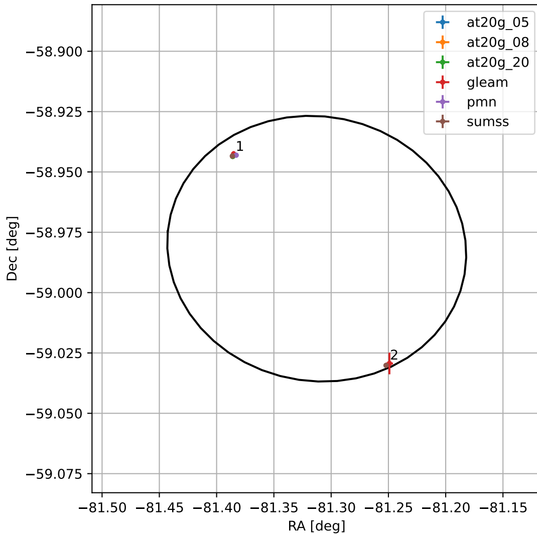
4FGL J1834.7-5858
