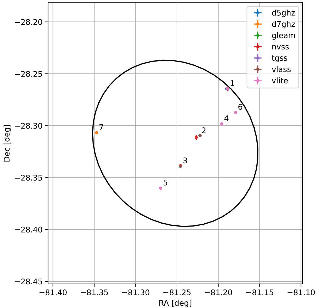
4FGL J1834.9-2819
