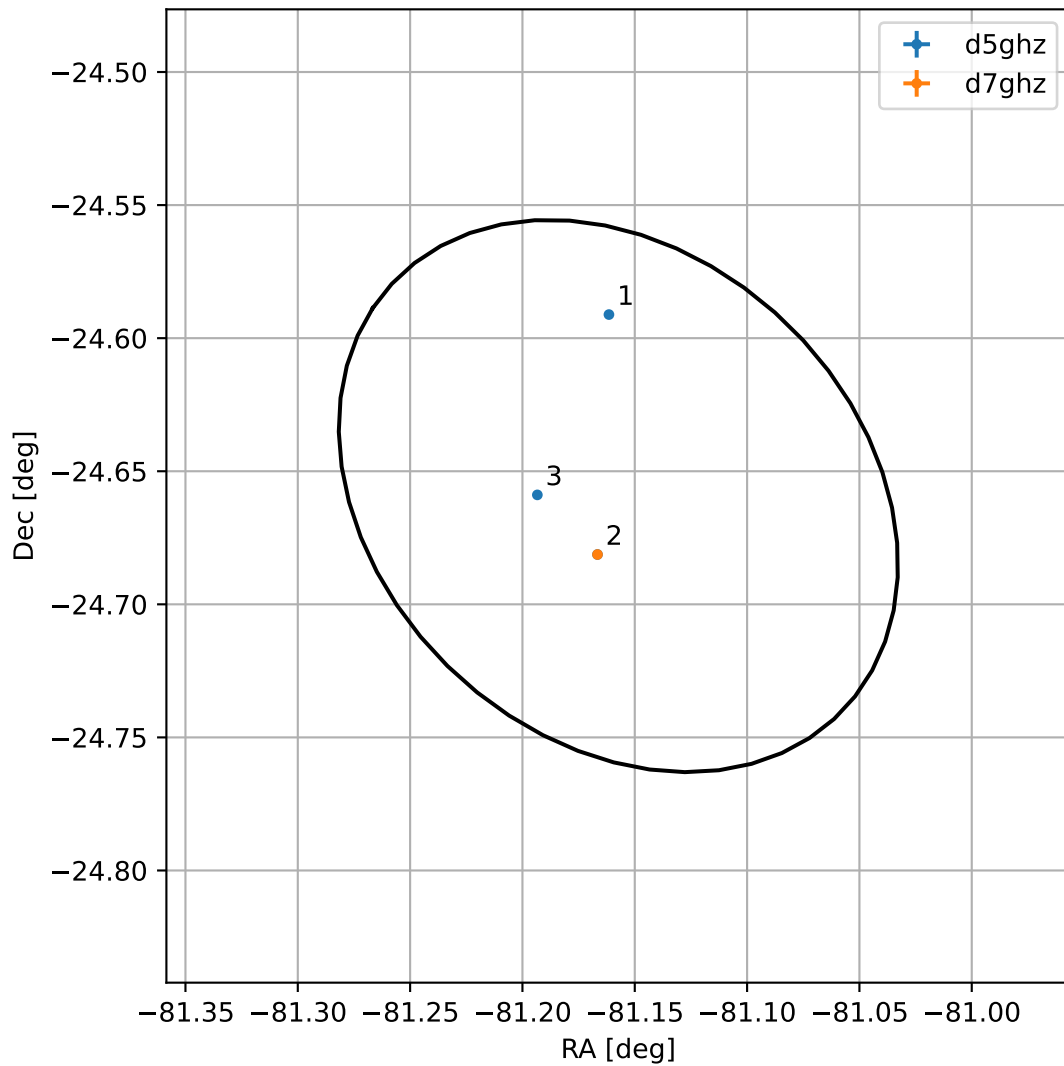
4FGL J1835.3-2439
