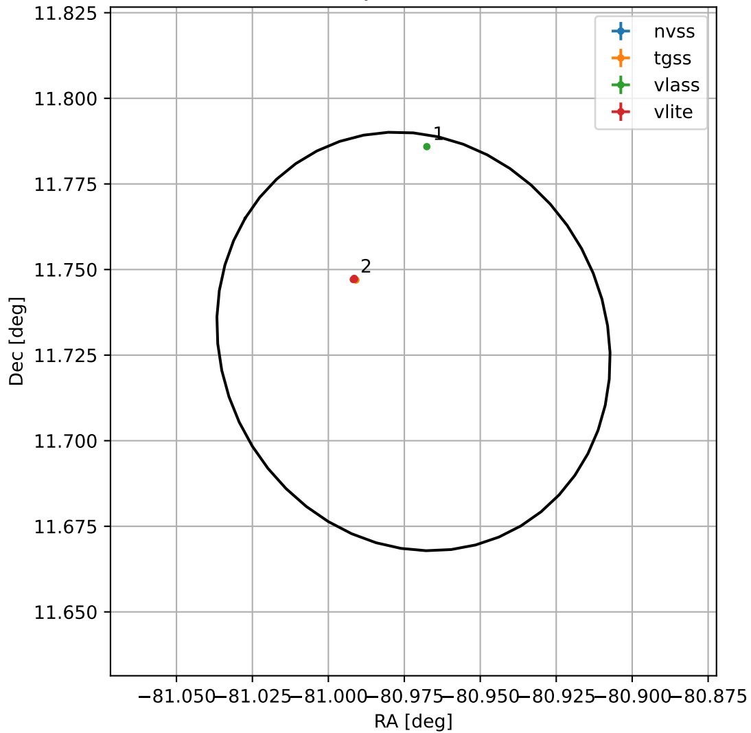
4FGL J1836.1+1143
