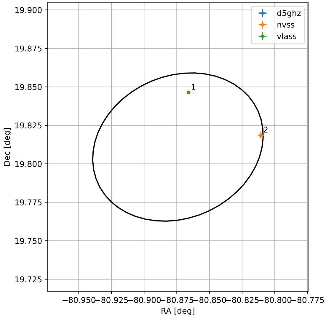
4FGL J1836.5+1948
