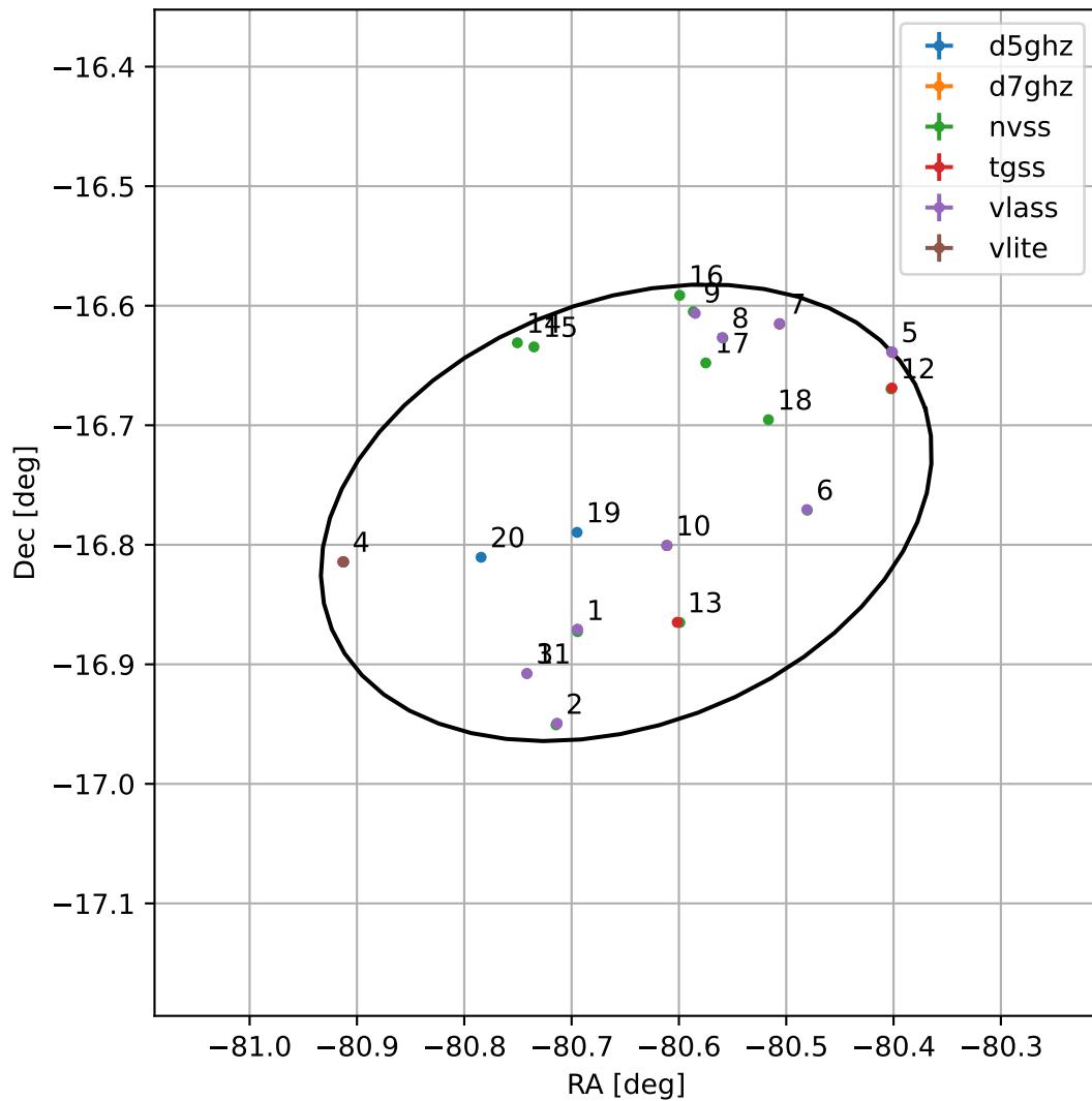
4FGL J1837.4-1646
