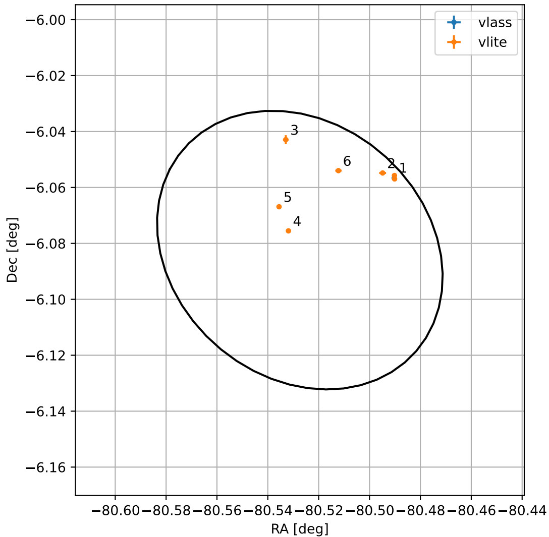
4FGL J1837.8-0604
