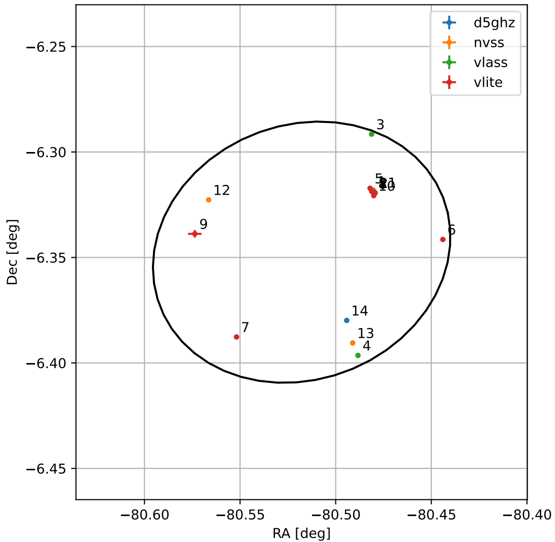
4FGL J1837.9-0620
