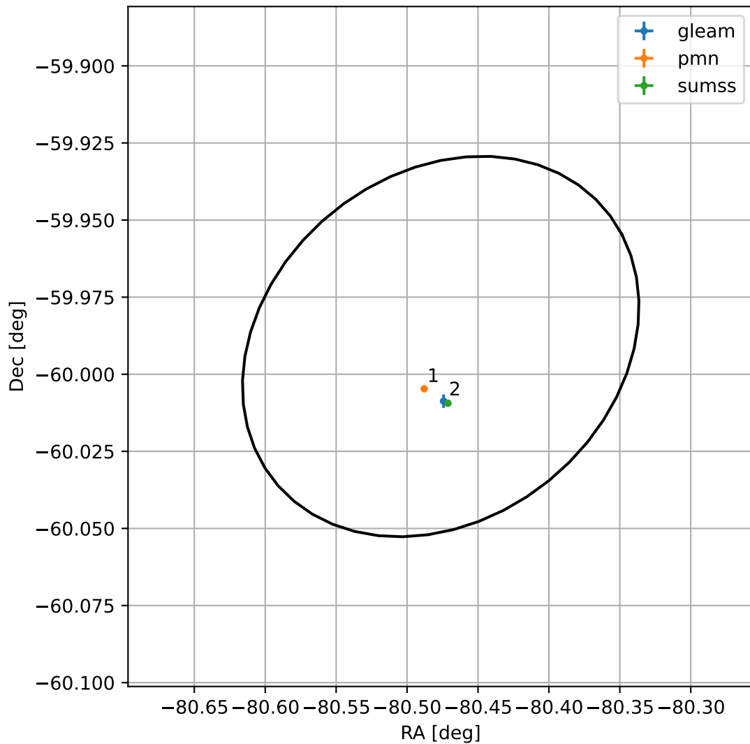
4FGL J1838.0-5959
