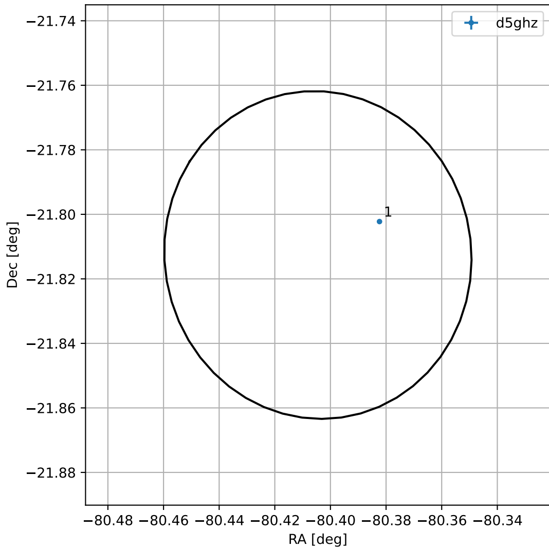
4FGL J1838.3-2148
