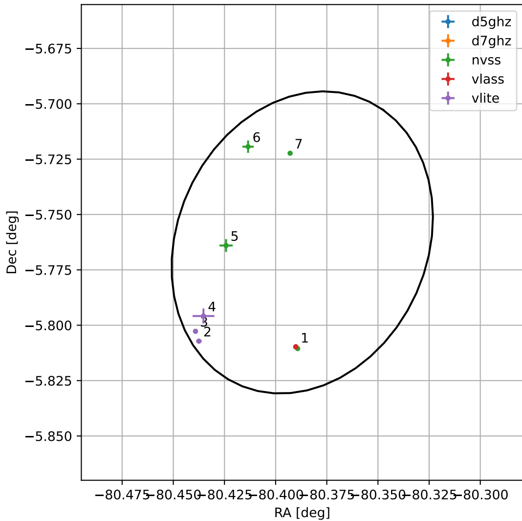
4FGL J1838.4-0545
