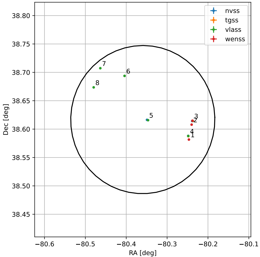
4FGL J1838.5+3837
