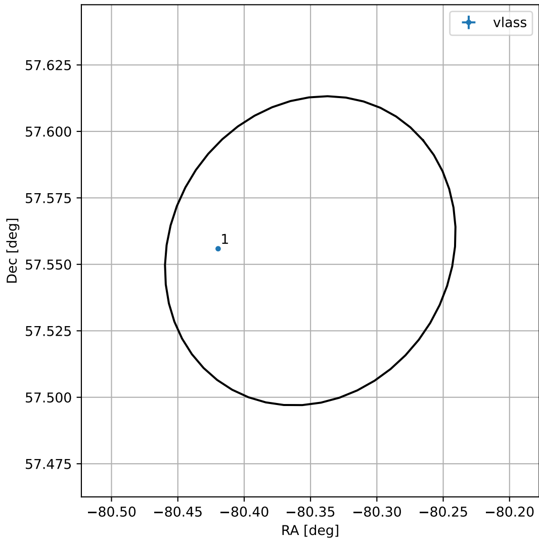
4FGL J1838.5+5733
