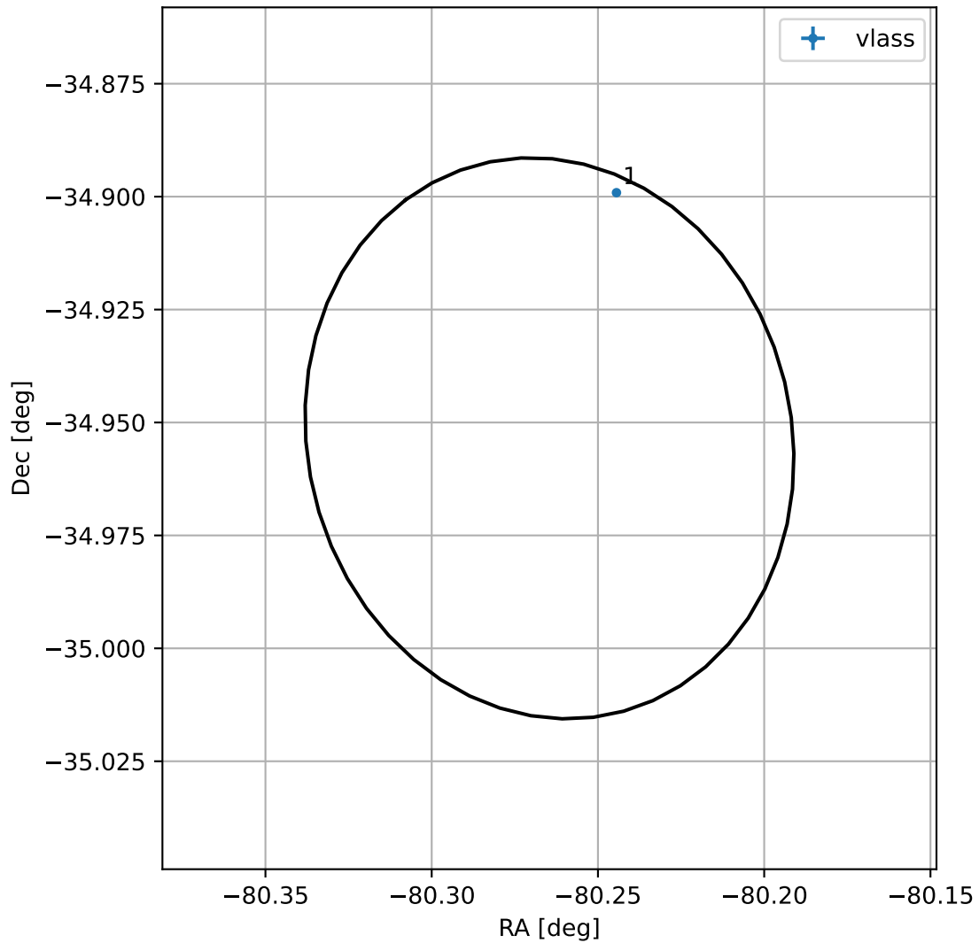
4FGL J1838.9-3457
