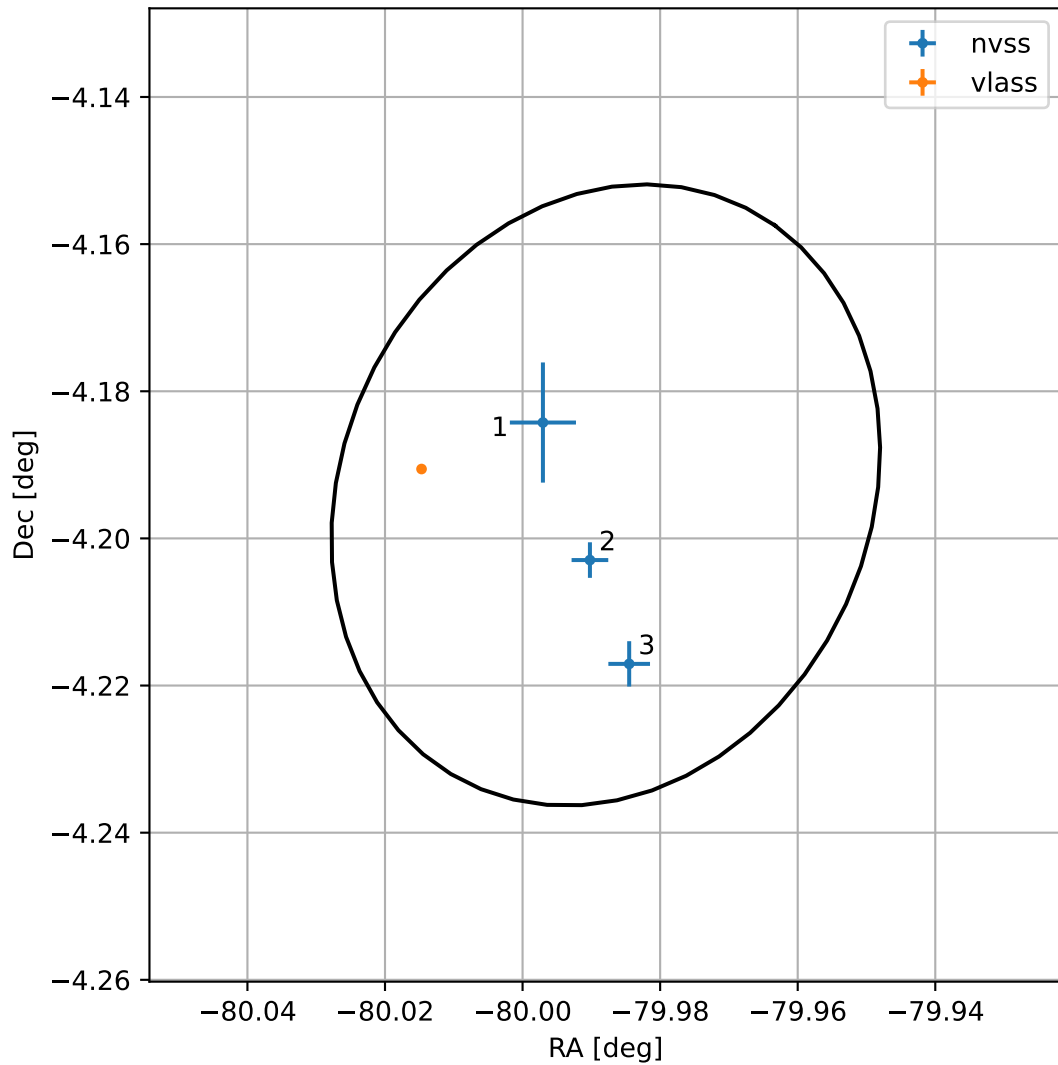
4FGL J1840.0-0411
